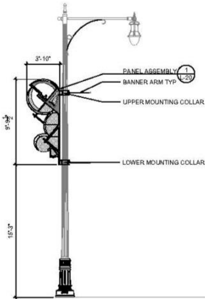
1 LIGHTPOLE GATEWAY 1 (QTY: 5) SCALE=1/8"=1'-0"
